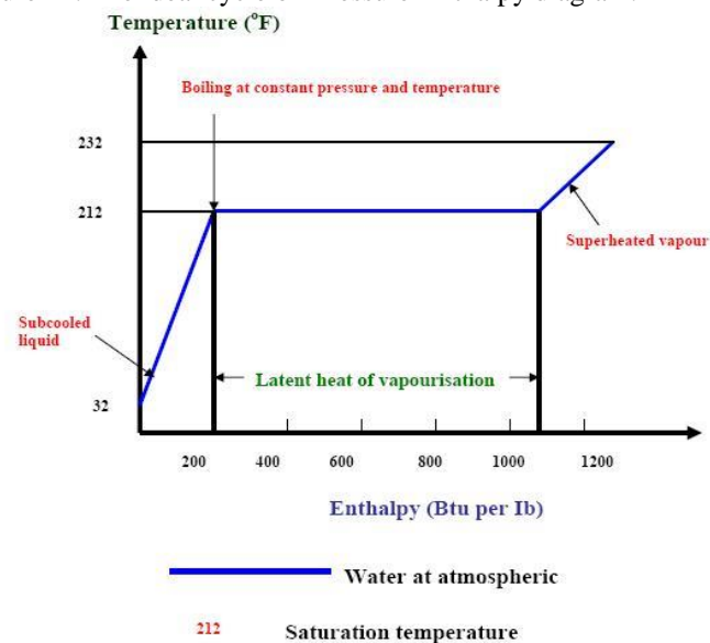
Figure 13. Water undergoing a change of state.
