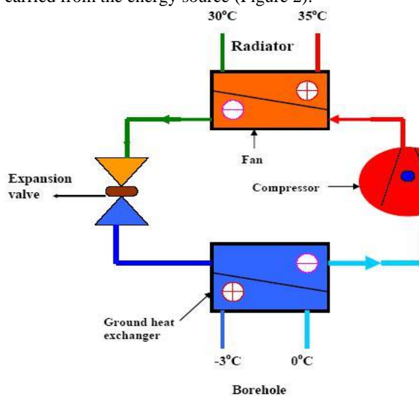
Figure 2. Detail of the GSHP circuit.
