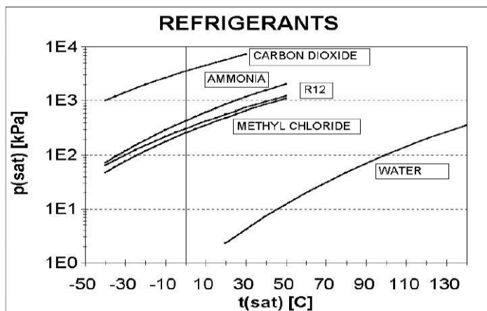
Figure 9. Refrigerant chart.
