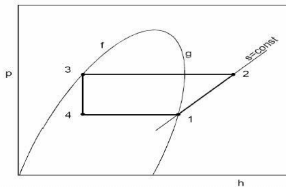
Figure 14. Refrigeration cycle.
