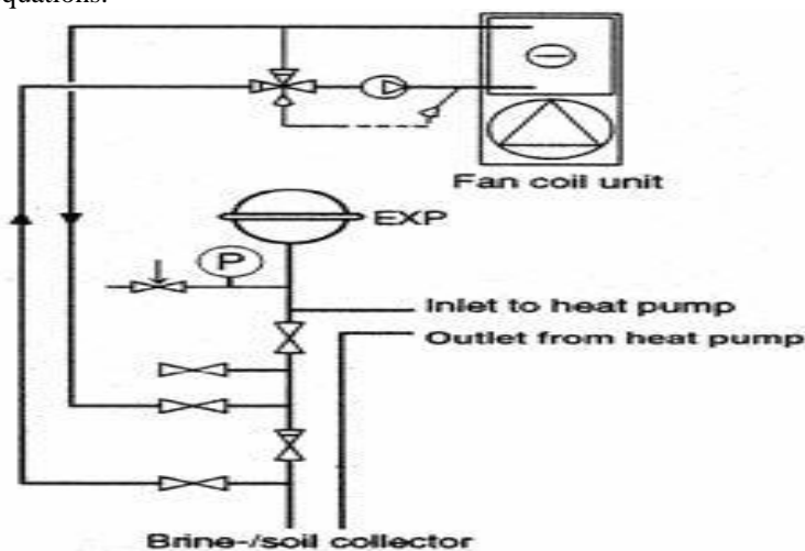
Figure 3. Diagram of cooling system.
