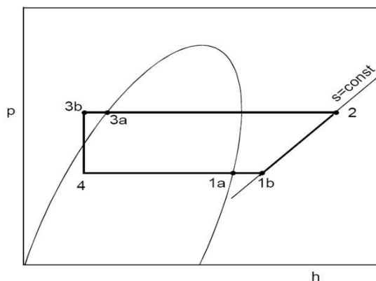
Figure 19. Diagram of liquid-suction heat exchanger.
