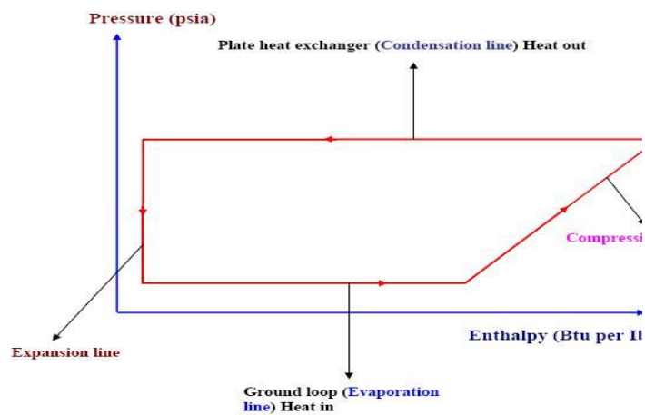
Figure 12. The ideal cycle on Pressure-Enthalpy diagram.
