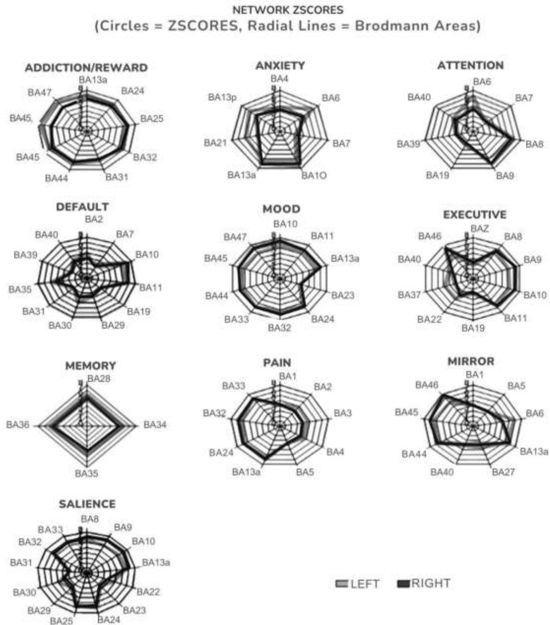
Figure 3. Post-intervention z-scores for specific Brodmann areas grouped by associated cognitive function, taken from report generated by Applied Neuroscience, Inc.
