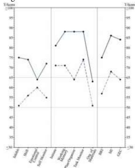
Figure 1. BRIEF-A Results
