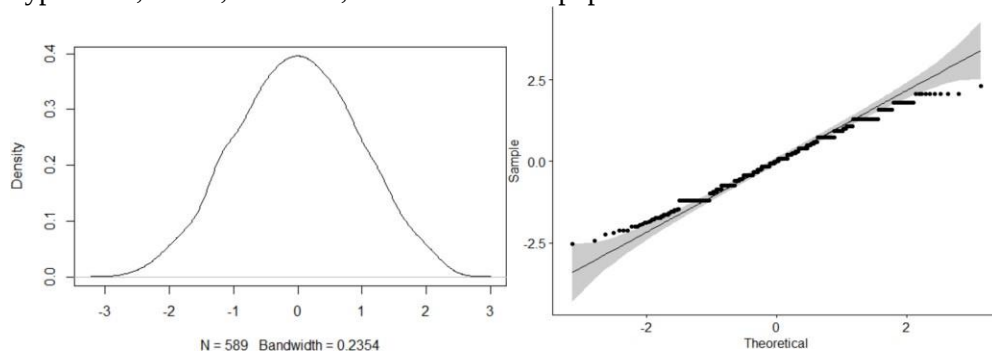
Figure 4: Checking the normality assumption for these data Table 2: Bartlett test of homogeneity of variances
