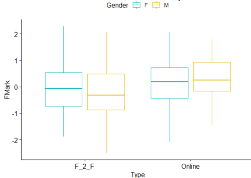
Figure 6: Boxplot chart of gender-based differences in student performance in the introductory computer science course across the delivery modes
