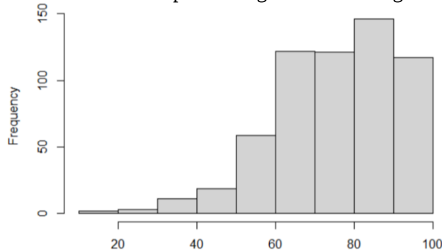
Figure 2: Histogram of student performance before data transformation
