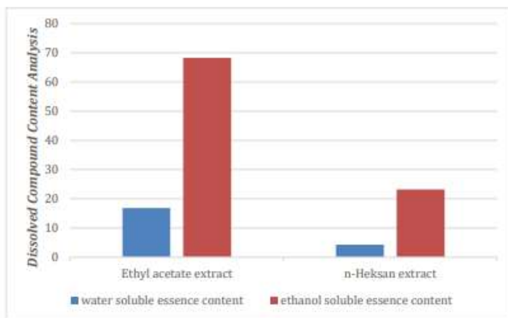
Figure 1. Dissolved Compound Content Analysis was Water soluble essence content (%) and Determination of ethanol soluble essence content (%) ethyl acetate Extract and n-Hexan Extract of Neem Leave
