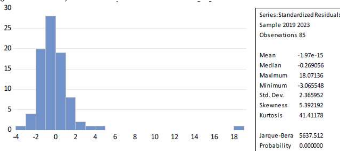
Figure 1 Normality Test
