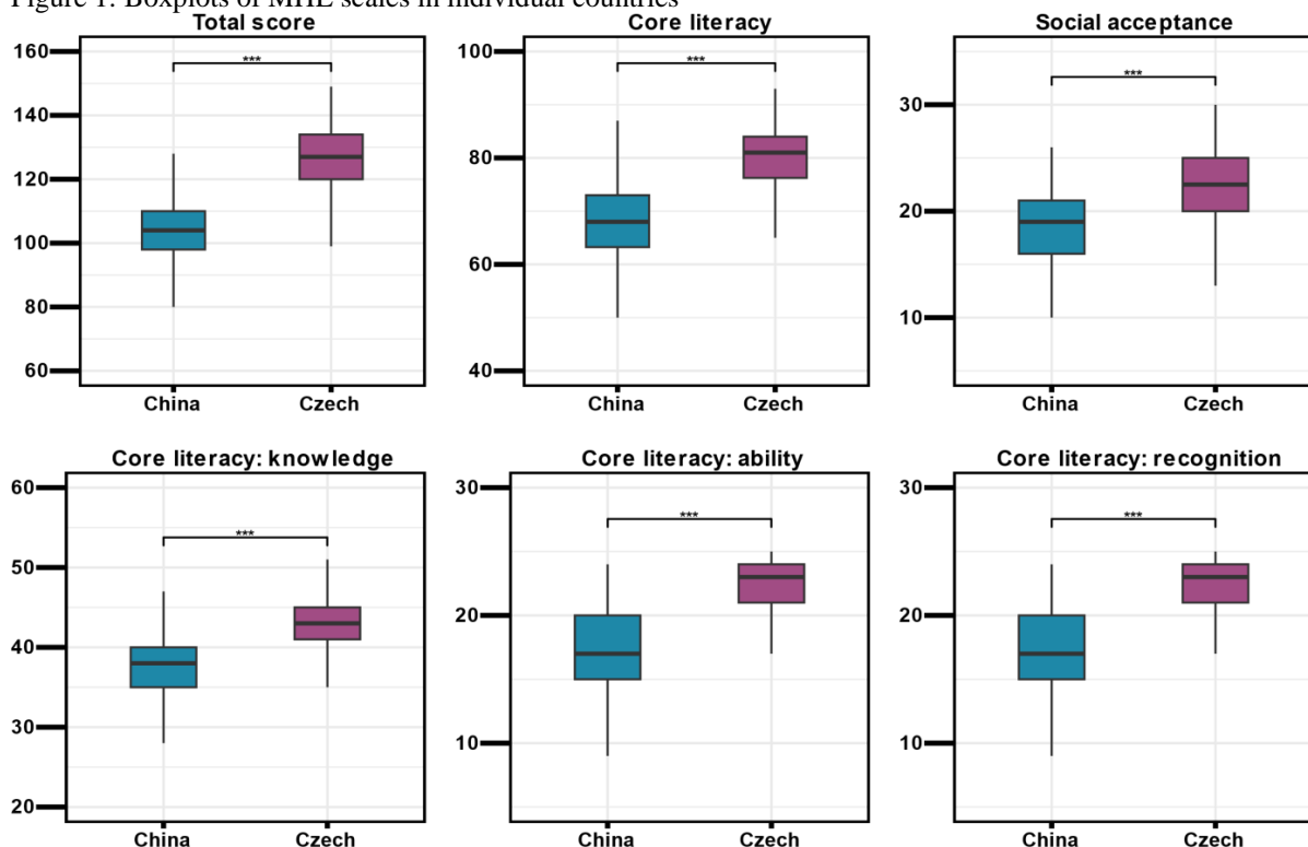
Figure 1: Boxplots of MHL scales in individual countries
