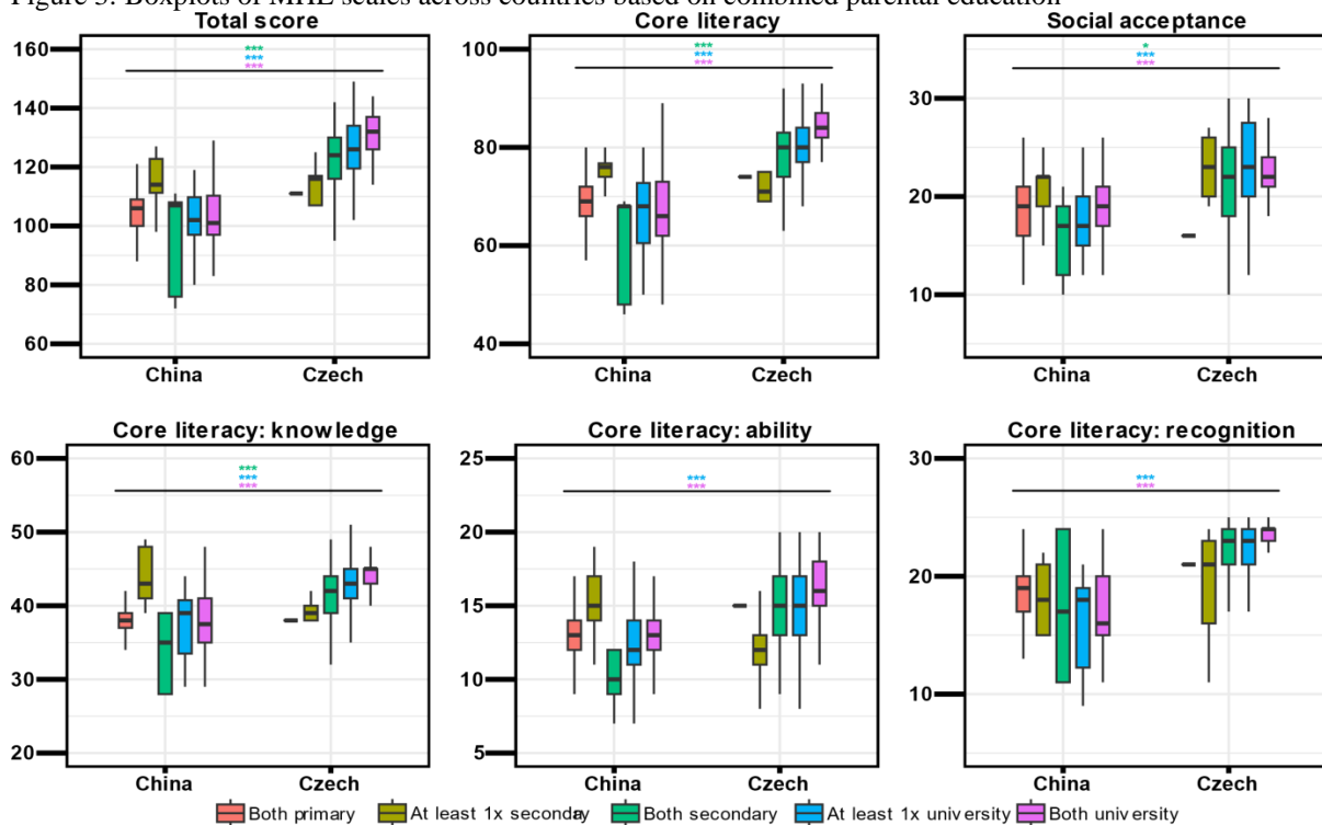
Figure 3: Boxplots of MHL scales across countries based on combined parental education
